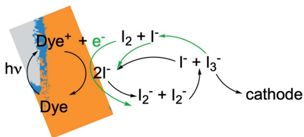
Fig. 10 Schematic of the electrolyte reactions involved in reduction of \text{Dye}^+ . The paths indicated by black arrows correspond to Sc3. The green arrows show how the \text{I}_2 –electron recombination reactions from Sc1 and Sc2 are coupled to them.
