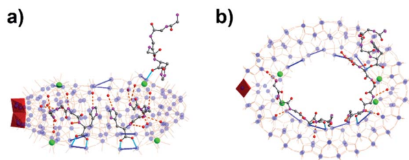
Fig. 4 (a) Side view and (b) top view of molecular structure of \{\text{Mo}_{126}\text{Ce}_4(\text{G}_4\text{H})_3\} , red polyhedron = \{\text{Mo}_2\text{O}_8\} . Color code is identical to that in Fig. 1.
