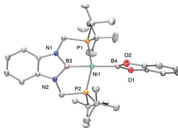
Fig. 1 Molecular structure of 3 (H atoms omitted for clarity). Thermal ellipsoids are represented at the 50% probability level. Selected bond distances (Å) and angles ( ^\circ ): \text{Ni}(1)\text{--B}(4) = 2.015(2) ; \text{Ni}(1)\text{--B}(3) = 1.942(2) ; \text{P}(1)\text{--Ni}(1)\text{--P}(2) = 157.74(3) ; \text{B}(3)\text{--Ni}(1)\text{--B}(4) = 175.0(1) .
