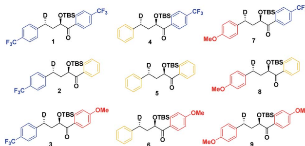
Fig. 4 Anti substrates for a NY-II reaction.
