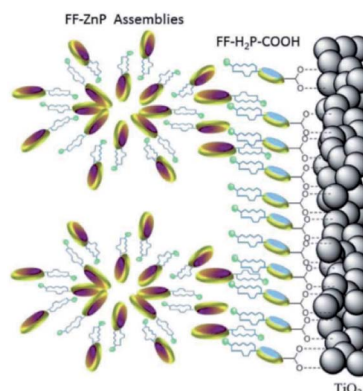
Fig. 31 Supramolecular antenna complexes are assembled onto n-type semi-conductors ( TiO_2 ) using hydrogen-bonding interactions. H_2 -porphyrin acceptor (blue discs) act as the seed for the growth of Zn-porphyrin antennae acting as energy donor. Used with permission from ref. 126.
