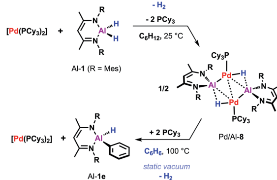
Scheme 7 (a) Pd-catalysed C–H alumination of benzene with Al-1. (b) Stoichiometric reactivity of [Pd(PCy 3 ) 2 ] with Al-1.
