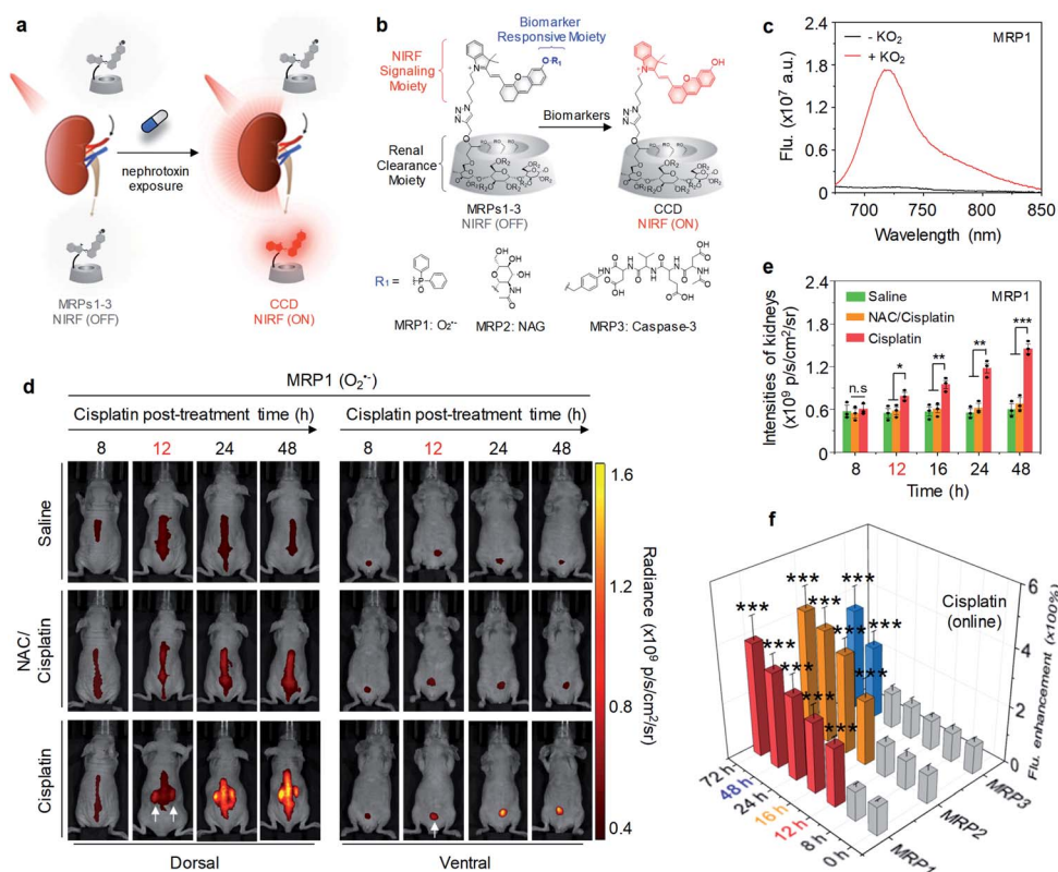
Fig. 5 (a) Schematic illustration of NIRF imaging of drug-induced AKI using MRPs1–3. (b) Chemical structures and molecular mechanisms of MRPs1–3 and their activated forms in response to O 2 •- , NAG and caspase-3, respectively (R = H or CH 2 CHOHCH 3 ). (c) Fluorescence spectra of MRP1 (30 μM) in the absence or presence of KO 2 (60 μM) in PBS buffer (10 mM, pH 7.4). (d) Representative NIR fluorescence images of living mice with injection of MRP1 after treatment of cisplatin (20 mg per kg body weight) for 8, 12, 24 or 48 h. The control groups were treated with PBS or a nephroprotective antioxidant NAC. NIRF images acquired at 720 nm upon excitation at 675 nm. (e) NIRF intensities of kidneys in living mice after 30 min injection of MRP1 at the different post-treatment time points (8, 12, 16, 24 or 48 h). (f) Fluorescence enhancement of excreted MRPs1–3 in the urine from cisplatin-treated living mice after injection at different time points post-treatment of cisplatin. n.s.: not significant, * p < 0.05, ** p < 0.01, *** p < 0.001. Reproduced with permission from ref. 56. Copyright 2019 Springer Nature.
