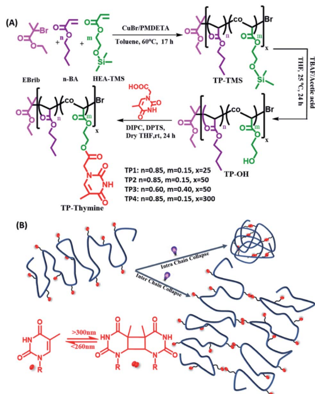
Scheme 1 (A) Synthetic scheme for the thymine functionalized polymers possessing different functionalities% and degree of polymerizations. (B) Schematic representation of the polymers undergoing homo-functional intra and interchain collapse by means of reversible photodimerization of thymine.
