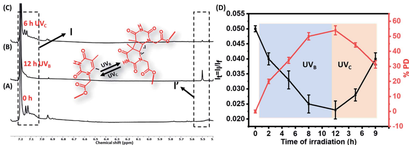
Fig. 2 Monitoring photodimerization of the polymers 1 H NMR. Stacked partial 1 H NMR spectra of the polymer TP1 (A) before and (B) after 12 h irradiation of UV B to form di-TP1, a [2\pi + 2\pi] cyclobutane adduct. (C) Partial 1 H NMR spectra of the polymer TP1 after 6 h irradiation of UV C . (D) Graph showing the change in the integral ratio of the protons of thymine moiety (black line) and photodimerization% degree (red line) with time course of UV B and UV C irradiations.
