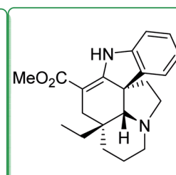
136 : (+)-Vincadifformine
