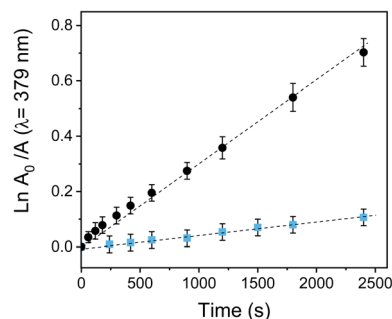
Fig. 5 First-order kinetic data fitting for the photooxidation of DMA in DMF sensitized by PEDOT-C 60 (■) and fullerene C 60 (●). \lambda_{irr} = 455-800 nm. Values represent mean \pm standard deviation (error bars) of three consecutive experiments.
