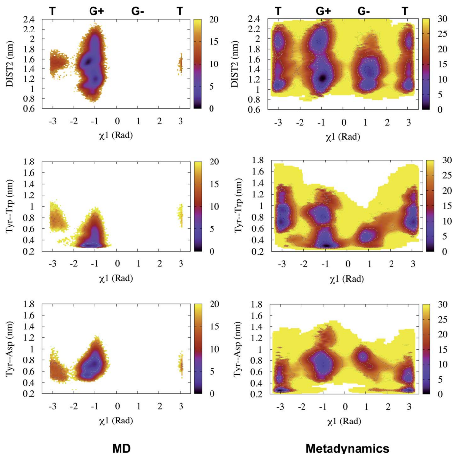
Fig. 10 Sampling of \chi_1 and DIST2 order parameters in MD (~600ns) and metadynamics simulations starting with apo PlmII (PDB ID:1LF4). The open flap conformation centres around DIST2 \sim 2.0 nm. The gauche + conformation was stabilised by H-bond interaction between Tyr and Trp whereas the trans conformation was stabilised by H-bond interaction between Tyr and catalytic Asp. The typical H-bond distance is 0.3–0.35 nm. z axis in the contour plot shows apparent free energy in \text{kJ mol}^{-1} .
