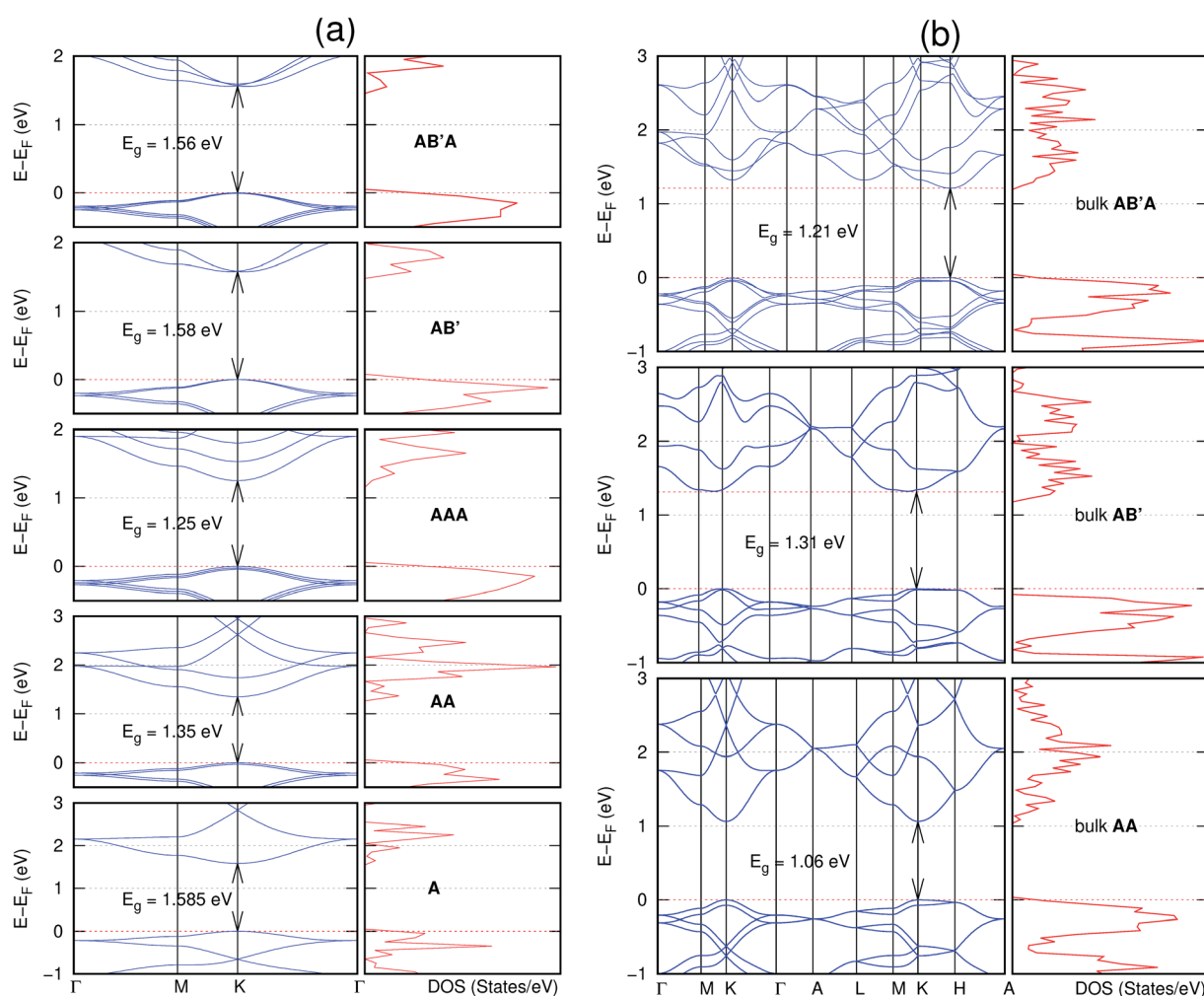
Fig. 6 Effect of stacking on the electronic structure of C_6N_6 -h2D for (a) isolated one, two, and three layers with the specified stackings and (b) the bulk system with the specified stackings. The fundamental band gap is marked with an arrow that indicates their direct nature. The stacking AB' indicates that the most stable stacking corresponds to neither AA nor AB. The Fermi level is set at the top of the valence band.
