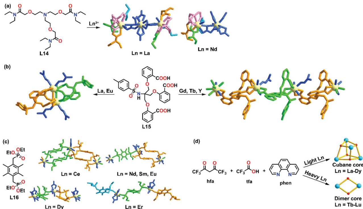
Fig. 3 Cationic radii-dependent supramolecular formation of (a) L14, reproduced with permission from ref. 42. Copyright 2003 American Chemical Society, (b) L15, reproduced with permission from ref. 43. Copyright 2010 The Royal Society of Chemistry, (c) L16, reproduced with permission from ref. 44. Copyright 2011 The Royal Society of Chemistry and (d) a series of cubanes and cluster reported by our group, reproduced with permission from ref. 45. Copyright 2018 American Chemical Society.
