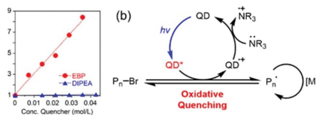
Fig. 5 (a) Stern–Volmer plot of QD fluorescence ( \lambda_{\text{ex}} = 460\text{ nm} ) effectively quenched by EBP but not by DIPEA. (b) Proposed oxidative quenching mechanism of ATRP catalyzed by CdSe QDs. Reproduced from ref. 61 with permission from the American Chemical Society, copyright 2018.
