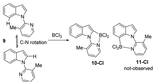
Scheme 5 3-Methyl pyridine directed C-H borylation of indole at C2.
