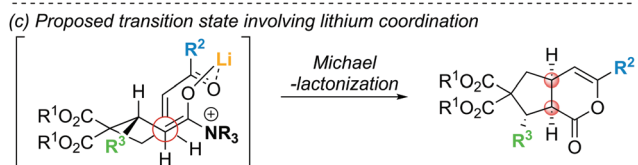
Scheme 21 (a) Michael–Michael-lactonization cascade for the synthesis of cyclopentanes; (b) kinetic analysis using an Eyring plot; (c) substrate organisation in transition state.
