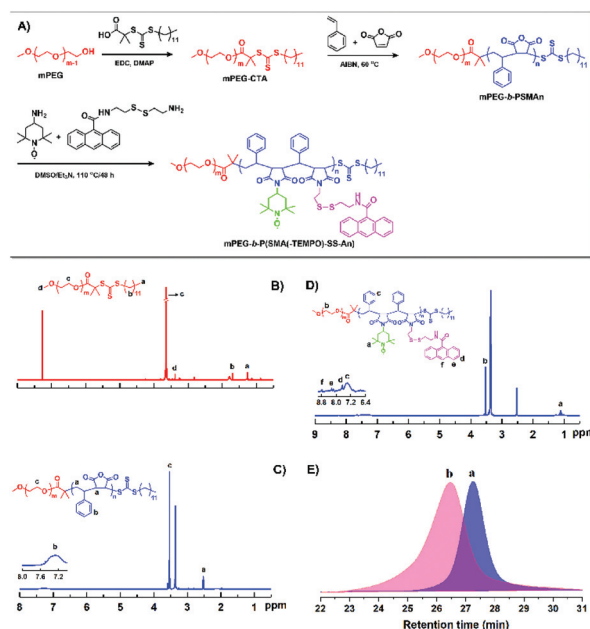
Fig. 1 Schematic illustration of the synthetic route (A) and characterization of mPEG- b -P(SMA(-TEMPO)-SS-An). 1 H NMR spectra of mPEG-RAFT macro-CTA in CDCl 3 (B), mPEG- b -PSMAAn in DMSO-d 6 (C) and mPEG- b -P(SMA(-TEMPO)-SS-An) in DMSO-d 6 (D), and (E) GPC traces of the polymers of mPEG-RAFT (a) and mPEG- b -PSMAAn (b) with THF as an eluent.
