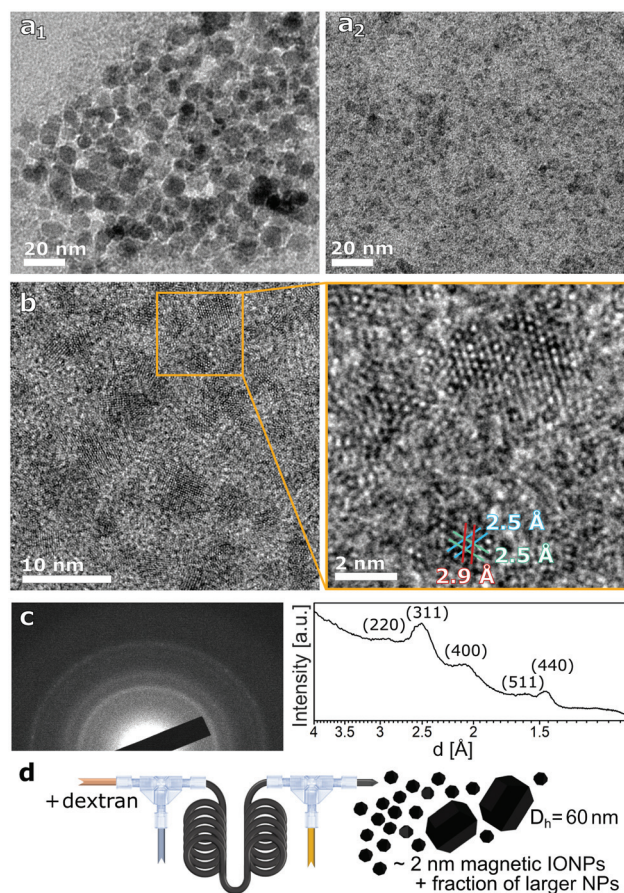
Fig. 2 Analysis of IONPs synthesised with dextran in the precursor solution and quenching 5 s after initiating co-precipitation. (a) TEM images of small fraction of particles >10 nm (a 1 ) and ultra-small IONPs (a 2 ). (b) HRTEM image of ultra-small IONPs with a higher magnification image matching the [111] zone axes of magnetite with the two 2.5 Å (113) planes and one 2.9 Å (220) plane. (c) Electron diffraction pattern (of the area in Fig. 2b) and the radially averaged diffraction profile matching the pattern of magnetite (PDF ref. 03-065-3107). (d) Schematic of flow synthesis in the presence of dextran.
