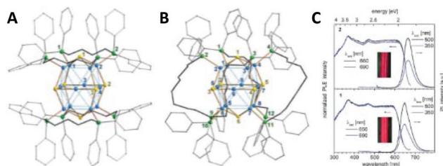
Fig. 7 Molecular structure of (A) [\text{Cu}_{12}\text{S}_6(\text{dpptt})_4] and (B) [\text{Cu}_{12}\text{S}_6(\text{dppt})_4] clusters. Colour codes of the elements: Cu: blue, S: yellow, P: green and C: grey. H atoms are omitted for clarity. (C) Room temperature photoluminescence excitation (PLE) and emission (PL) spectra of a suspension of freshly prepared microcrystals of [\text{Cu}_{12}\text{S}_6(\text{dpptt})_4] (down) and [\text{Cu}_{12}\text{S}_6(\text{dppt})_4] (up) in toluene, measured in the integrating sphere. The inset shows the colours of the suspensions of microcrystal under white LED light. Republished with permission from ref. 164. Copyright 2014 Royal Society of Chemistry.
