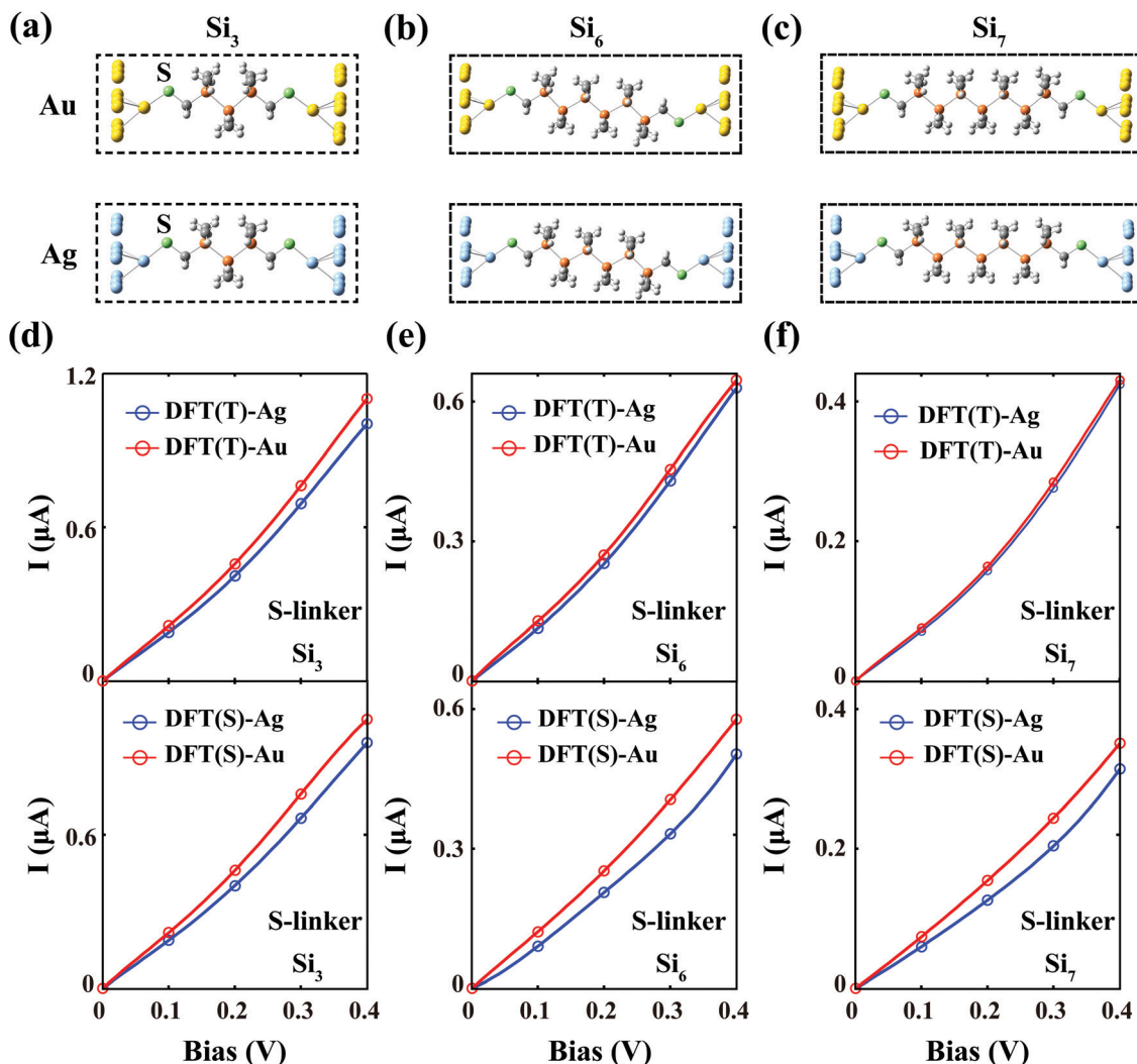
Fig. 2 I - V curves of the thiol-terminated silane junctions \text{Si}_n\text{-S-M} calculated from the DFT-based method. (a–c) The optimised atomic structures of \text{Si}_n\text{-S-M} ( \text{M} = \text{Au} or \text{Ag} ) are shown in (a) for n = 3 ( \text{Si}_3 ), (b) for n = 6 ( \text{Si}_6 ) and (c) for n = 7 ( \text{Si}_7 ). (d–f), I - V curves calculated from two DFT-based packages, TranSIESTA (DFT(T)) and SMEAGOL (DFT(S)), are shown in (d) for n = 3 , (e) for n = 6 and (f) for n = 7 . DFT(T or S)-Au/Ag denotes TranSIESTA or SMEAGOL results for \text{Si}_n\text{-S-Au/Ag} . For all cases, the Au contact produces a higher conductivity than that of the Ag contact.
