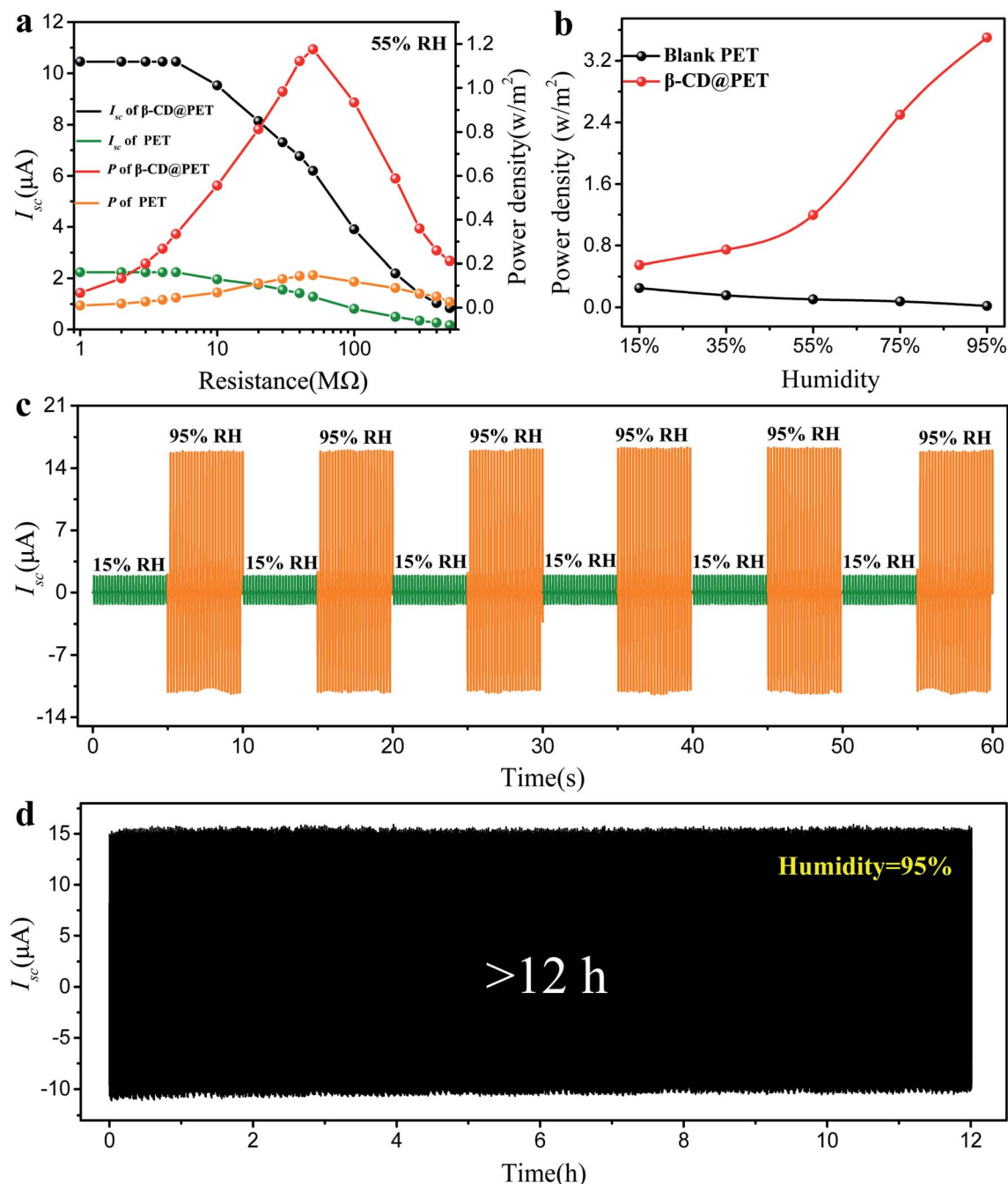
Fig. 4 Output performance, stability and reversible output performance of the β-CD@PET-based TENG. (a) Dependence of I_{sc} and the corresponding power density on the external loading resistance of blank PET- and β-CD@PET-based TENGs at a humidity of 55%, (b) comparison of the output power density of blank PET- and β-CD@PET-based TENGs at humidities from 15% to 95%, (c) reversible output properties of the β-CD@PET-based TENG in an alternating dry (RH 10%) and wet (RH 99%) environment, and (d) stability test of the β-CD@PET-based TENG at 95% RH.
