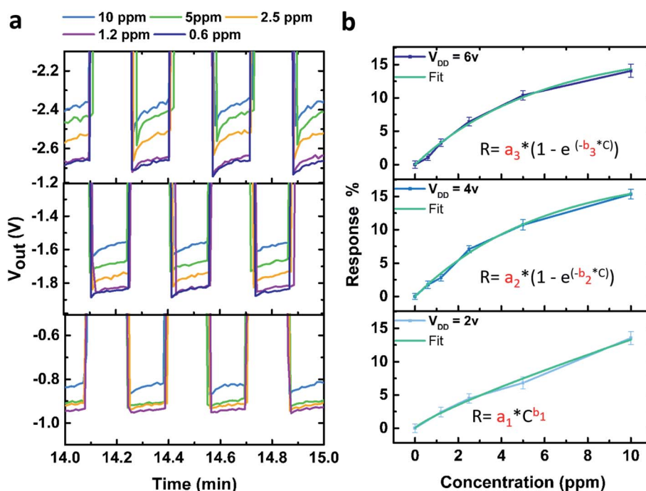
Fig. 3 (a) Output voltage of the inverter after exposure to various concentrations of NO 2 gas for a V_{\text{in}} at -4 V and -11 V alternatively for three different V_{\text{DD}} values (from top to bottom: V_{\text{DD}} = 6 V, 4 V and 2 V). (b) Response of the inverter as a function of NO 2 concentration for the three different V_{\text{DD}} values (from top to bottom: V_{\text{DD}} = 6 V, 4 V and 2 V).
