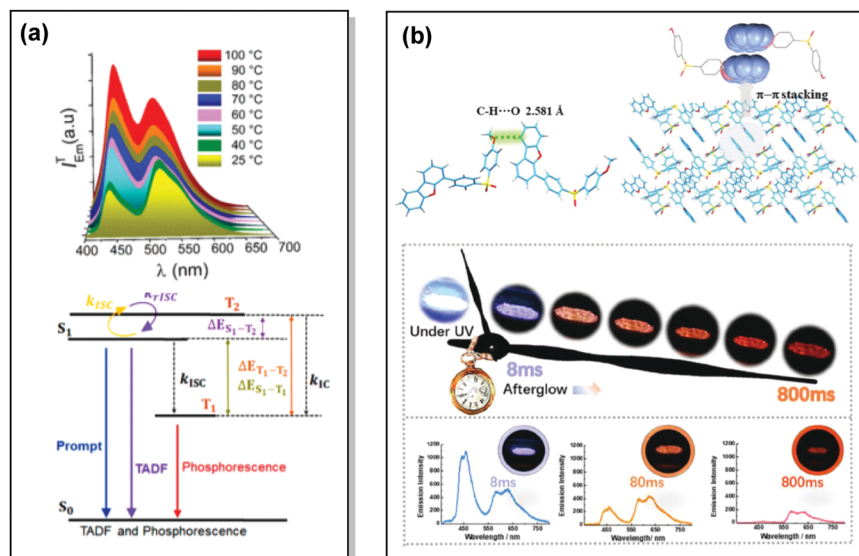
Fig. 17 Examples of DF/RTP dual emission in the systems with (a) monomer-type RTP (48) and (b) aggregate-type RTP (51). (a) Steady-state PL of 48 spectra upon heating from 25 to 100 °C; Jablonski diagram for DE via TADF and phosphorescence in the proposed molecular design (48). Reproduced with permission. 5 Copyright 2018 American Chemical Society. (b) Single crystal structure of 51 and \pi - \pi stacking properties of 51 in the single-crystal structure; emission photos of 51 during the afterglow emission processes; afterglow emission spectra of 51 at 8, 80, and 800 ms along with emission photos in ambient conditions. Reproduced with permission. 107 Copyright 2019 Wiley-VCH.
