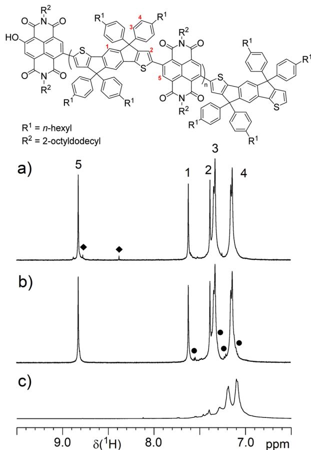
Fig. 1 ^1\text{H} NMR spectra of (a) P7 and (b) P6 . (c) depicts the ^1\text{H} NMR spectrum of model compound \text{Ph}_8\text{-PIDT} . Squares and dots mark signals of the -\text{NDI}-\text{OH} and the -\text{IDT}-\text{H} end groups, respectively.
