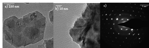
Fig. 2 TEM images (a) and (b). Diffraction of DPCOF spacing which corresponds to 2\theta 18–19°. The CTEM image displays clear hexagonal symmetry and crystalline order which can be seen in DPCOF SAD (c) diffraction from (b).
