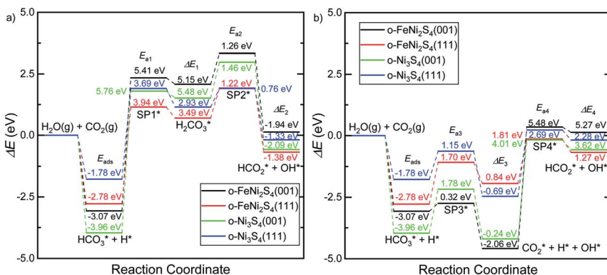
Fig. 5 Minimum energy pathways for CO 2 reduction by H 2 O via (a) substitution and (b) dissociation mechanisms on the (001) and (111) surfaces of the o-FeNi 2 S 4 and o-Ni 3 S 4 thiospinels. Minimum states and saddle points are denoted by horizontal lines linked by dashed lines. Energies are referenced to the isolated H 2 O and CO 2 molecules as well as the surface slab. Adsorbed species are denoted using the symbol *. Adsorption energies ( E_{\text{ads}} ), elemental step energies ( \Delta E_i ) and activation energies ( E_{\text{a}} ) are also indicated.
