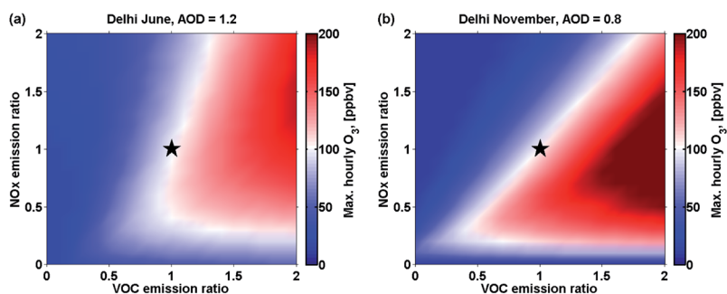
Fig. 3 Daily maximum hourly ozone in Delhi as a function of NO x and VOC emissions in (a) summer (June) and (b) winter (November). Current conditions are marked by a black star.
