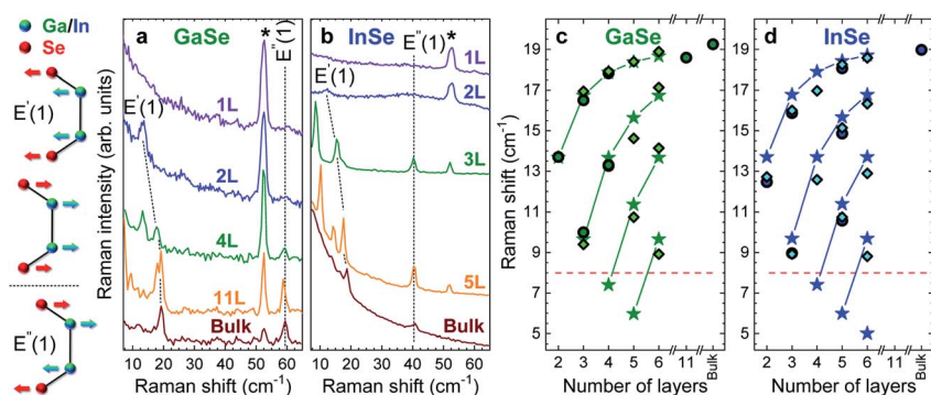
Fig. 5 Atomic displacements of phonon modes and unpolarized 514.5 nm low-frequency Raman spectra as a function of N for (a) GaSe and (b) InSe. Dashed lines are guides to the eye. (c and d) N dependence of C modes of (c) GaSe and (d) InSe. Circles and diamonds denote experimental results. Stars are DFT calculations. Dashed red horizontal lines represent the minimal Raman shift \sim 8 \text{ cm}^{-1} detectable in our experiments.
