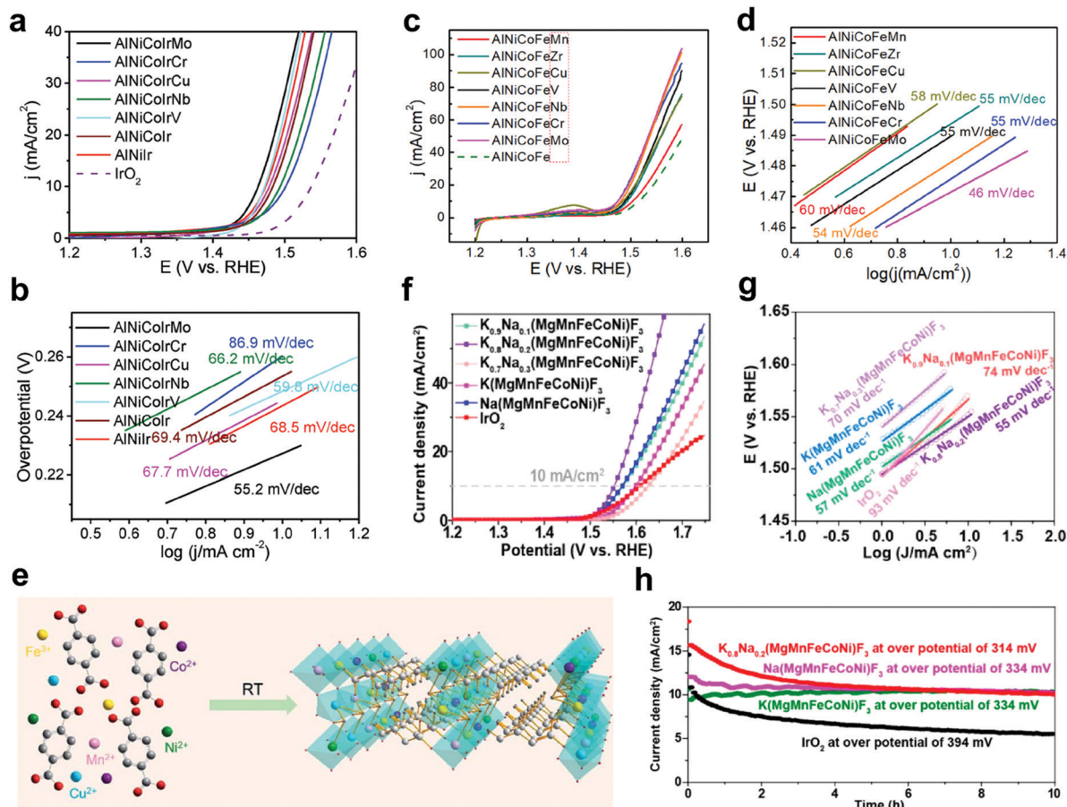
Fig. 6 (a) Linear sweep voltammetry and (b) the corresponding Tafel curves of different AlCoNiIr-based HEAs and \text{IrO}_2 in 0.5 M \text{H}_2\text{SO}_4 solution. Reproduced with permission. 39 Copyright 2019, Wiley-VCH. (c) Linear sweep voltammetry and (d) the corresponding Tafel curves for different AlCoNiFe-based HEAs in 1 M KOH solution. Reproduced with permission. 41 Copyright 2019, American Chemical Society. (e) Synthetic procedure for the preparation of MnFeCoNiCu-based HE-MOF at ambient conditions. Reproduced with permission. 42 Copyright 2019, The Royal Society of Chemistry. (f) Linear sweep voltammetry and (g) the corresponding Tafel curves as well as (h) chronoamperometric recording of \text{IrO}_2 and \text{Na}_x\text{K}_{1-x}(\text{FeCoNiMnMg})\text{F}_3 in 1 M KOH solution. Reproduced with permission. 43 Copyright 2020, American Chemical Society.
