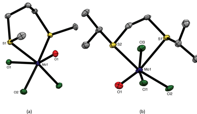
Fig. 1 Crystal structures of fac -[MoOCl 3 {MeS(CH 2 ) 3 SMe}] (a) and mer -[MoOCl 3 {iPrS(CH 2 ) 2 S i Pr}] (b) showing the atom numbering scheme. Ellipsoids are shown at 50% probability, hydrogen atoms omitted for clarity. Selected bond lengths (Å) and angles (°): (a) Mo1–Cl1 = 2.4540(2), Mo1–Cl2 = 2.3451(2), Mo1–Cl3 = 2.3451(4), Mo1–O1 = 1.674(1), Mo1–S1 = 2.5388(3), Cl1–Mo1–Cl2 = 94.52(2), Cl2–Mo1–Cl3 = 92.55(3), Cl2–Mo1–O1 = 101.87(4), Cl3–Mo1–O1 = 101.87(4), S1–Mo1–S1 = 97.95(2); (b) Mo1–Cl1 = 2.3578(8), Mo1–Cl2 = 2.3378(8), Mo1–Cl3 = 2.3618(7), Mo1–O1 = 1.671(2), Mo1–S1 = 2.8298(8), Mo1–S2 = 2.5665(7), Cl1–Mo1–Cl2 = 91.25(3), Cl1–Mo1–O1 = 98.99(8), Cl1–Mo1–Cl3 = 89.69(3), Cl2–Mo1–O1 = 98.99(8), S1–Mo1–S2 = 78.83(2).
