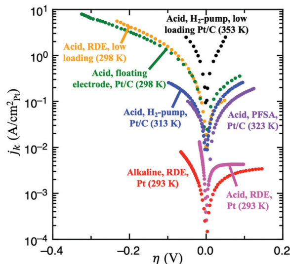
Fig. 4 Experimental results for HOR/HER utilizing several different experimental techniques. From lowest to highest specific current: full sized Pt RDE in \text{H}_2 -saturated 0.1 M KOH, 10 \mu\text{g}_{\text{Pt}} \text{cm}_{\text{disk}}^{-2} , 3600 rpm, 10 \text{ mV s}^{-1} (red, ref. 9); full sized Pt RDE in \text{H}_2 -saturated 0.1M \text{HClO}_4 , 3600 rpm (pink, ref. 9); Pt/C dispersed on an Au grid in contact with a perfluorosulfonic acid (PFSA) membrane, 90 \text{ m}^2 \text{g}_{\text{Pt}}^{-1} , 5 \text{ mV s}^{-1} (purple, ref. 46); Pt/C using the \text{H}_2 -pump approach in a proton exchange fuel cell (PEMFC) setup, 2 \text{ mV s}^{-1} (blue, ref. 21); Pt/C in 4M \text{HClO}_4 using the floating electrode technique, 0.84 \mu\text{g}_{\text{Pt}} \text{cm}^{-2} , 10 \text{ mV s}^{-1} (green, ref. 18); low loading Pt/C RDE in 0.5M \text{H}_2\text{SO}_4 , 13 \text{ ng}_{\text{Pt}} \text{cm}^{-2} , 1600 rpm, 50 \text{ mV s}^{-1} (yellow, details in ref. 8); and low loading Pt/C using the \text{H}_2 -pump approach in a PEMFC, 3 \mu\text{g}_{\text{Pt}} \text{cm}^{-2} (black, details in ref. 19).
