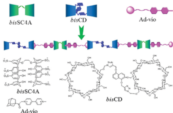
Scheme 24 Schematic representation of bisSC4A, Ad-Vio, bisCD and the supramolecular ternary polymer [bisCD]–[Ad-Vio]–[bisSC4A]. The scheme has been reproduced from ref. 110 with permission from the Royal Society of Chemistry.
