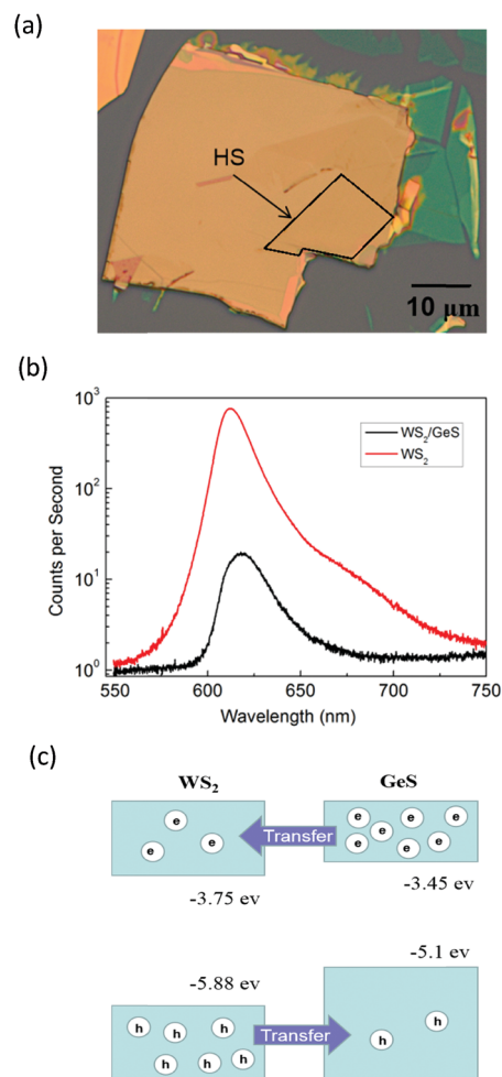
Fig. 3 (a) Optical microscope image of the WS 2 /GeS heterostructure; the heterostructure is in the black box. (b) Photoluminescence spectra of the samples measured from the regions of monolayer WS 2 (red) and the heterostructure (black). (c) The predicted band alignment of the WS 2 /GeS heterostructure.
