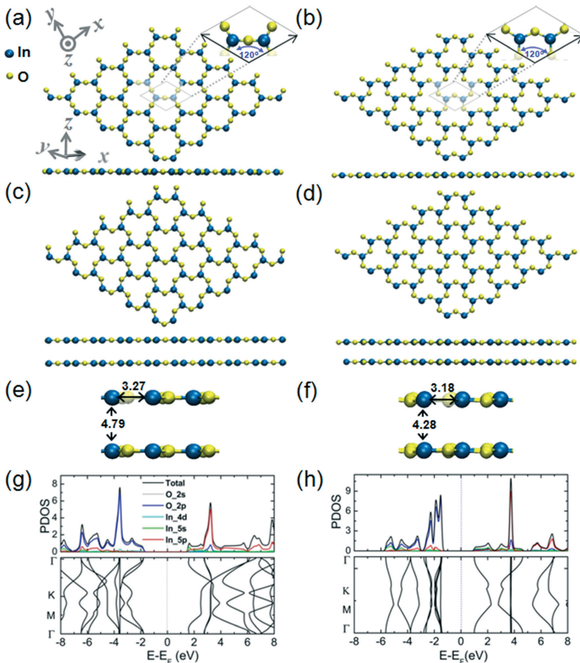
Fig. 2 Structure of a h-In 2 O 3 monolayer from top and side views (a), the relaxed bilayer structure from top and side views (c), and a magnified side view of the bilayer structure (e) with characteristic atomic distances indicated. The unit cell is depicted in (a). This unit cell comprises two In atoms and three O atoms, the lengths of the \vec{a} and \vec{b} cell vectors reading |\vec{a}| = |\vec{b}| = 5.85 \text{ \AA} , with an angle between them of 120 degrees. Plots of partial density of states (PDOS) and band structure are shown in (g). Structure of an alternative h-In 2 O 3 monolayer featuring 12-membered rings from top and side views (b), the relaxed bilayer structure from top and side views (d) and a magnified side view of the bilayer structure (f) with characteristic atomic distances indicated. The unit cell is depicted in (b). This unit cell comprises two In atoms and three O atoms, the lengths of the \vec{a} and \vec{b} cell vectors reading |\vec{a}| = |\vec{b}| = 6.36 \text{ \AA} , with an angle between them of 120 degrees. Plots of partial density of states (PDOS) and band structure are shown in (h).
