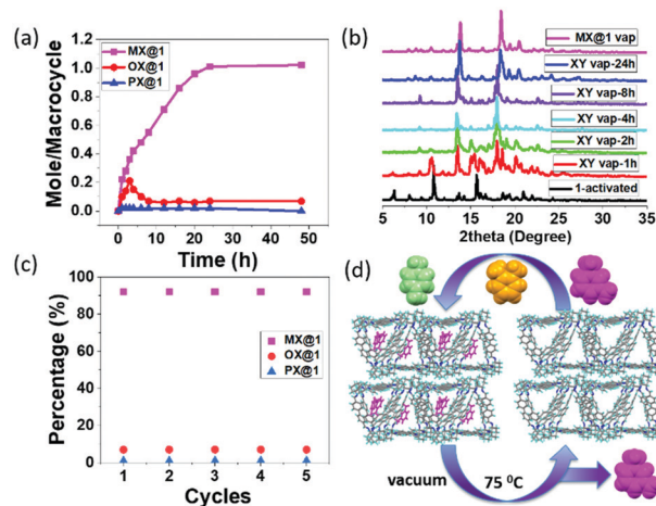
Fig. 4 (a) Solid–vapor sorption of 1 in OX/MX/PX (1:1:1 v/v) xylenes. (b) Time dependent PXRD of 1 to MX@a1 in the presence of OX/MX/PX (1:1:1 v/v) vapor. (c) Relative uptakes of MX after five recycles. (d) Schematic representation of MX release from MX@a1 to 1 upon heating and uptake of MX again from the mixture vapor.
