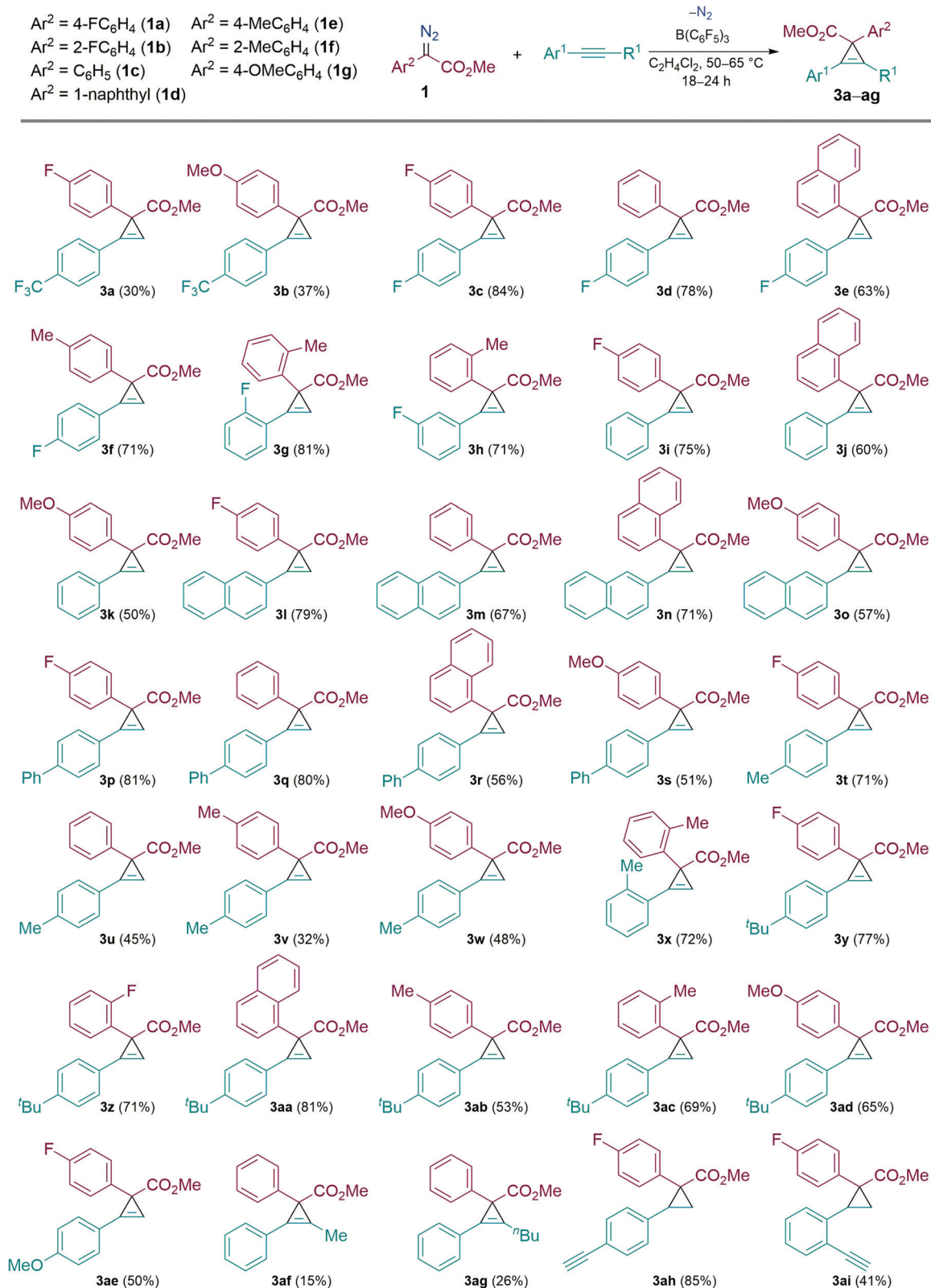
Scheme 2 Substrate scope for the cyclopropanation of arylalkynes. Yields reported are isolated. All the reactions were carried out in 0.1 mmol scale, 10 mol% \text{B(C}_6\text{F}_5)_3 was used. 1 (1.3 equiv.), phenylalkyne (1 equiv.), and 1.5 mL of solvents were used.
