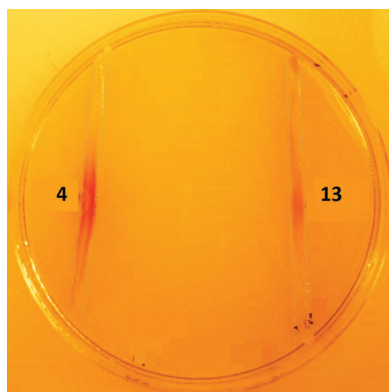
Fig. 3 Chemical complementation of S39006 \Delta pigD with aldehyde 4 (left) and thioester 13 (right).
