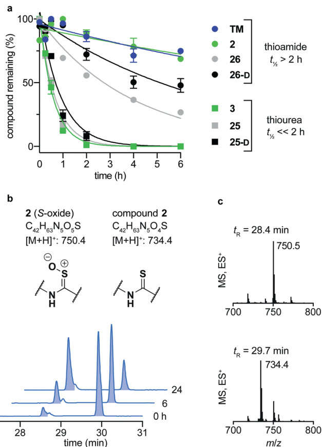
Fig. 5 Stability assays in human serum. (a) Stability assays of selected compounds in human male serum. (b) UV ( A_{280} ) and (c) TIC (ESI) chromatograms and mass spectra at relevant time points of compound 2 monitoring degradation in serum. Data are shown as mean values relative to the peak intensity at t = 0 h \pm SEM, n = 2-3 . For t_{1/2} values, see Table S7 (ESI † ).
