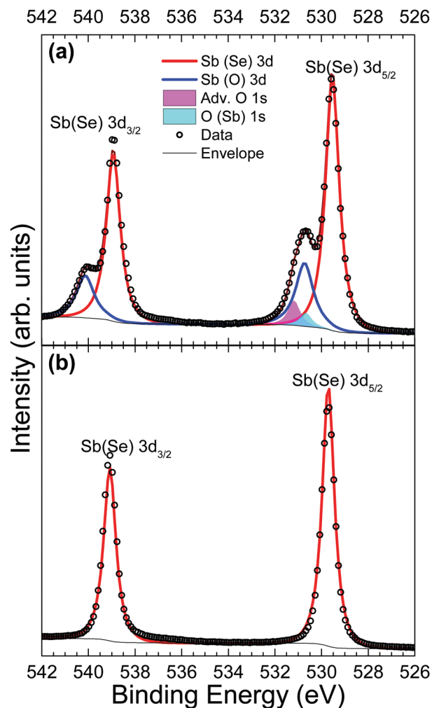
Fig. 3 Sb 3d HAXPES data from an \text{Sb}_2\text{Se}_3 crystal (a) before and (b) after in situ cleaving.
