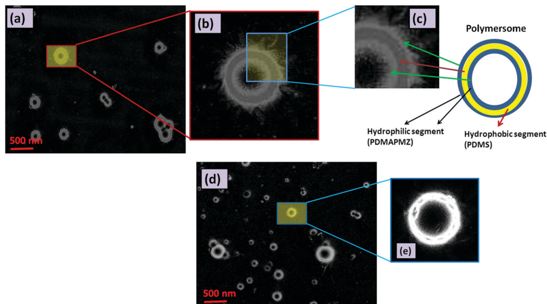
Fig. 3 HRTEM image of the (a) ZPDAPM- b -PDMS- b -ZPDAPM tri-block copolymer based polymersome; (b) and (c) magnified view of the polyzwitterionic polymersome; (d) amine modified PDMS tri-block copolymer (AmPGMA- b -PDMS- b -AmPGMA) based polymersome and (e) magnified view of the amine functionalized polymersome.
