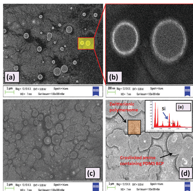
Fig. 4 FESEM images of the (a) ZPDAPM- b -PDMS- b -ZPDAPM tri-block copolymer based polymersome; (b) magnified view of the polymersome; (c) amine modified PDMS tri-block copolymer (AmPGMA- b -PDMS- b -AmPGMA) based polymersome; and (d) curcumin loaded polyzwitterionic polymersome incorporated PDMS- \text{NH}_2 crosslinked hydrogel and (e) elemental analysis of the hydrogel.
