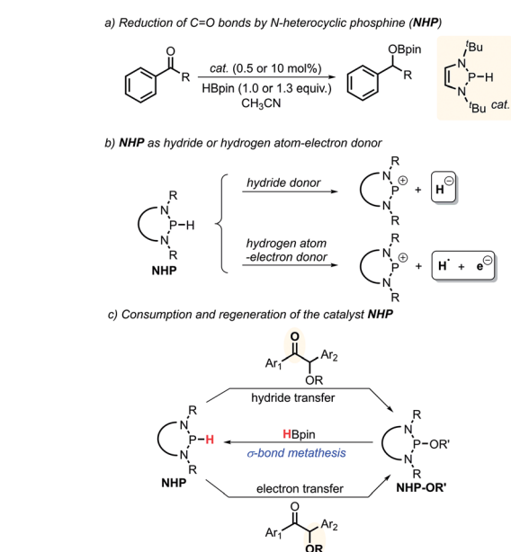
Scheme 2 Chemical transformations of N -heterocyclic phosphines NHPs in reduction reactions.
