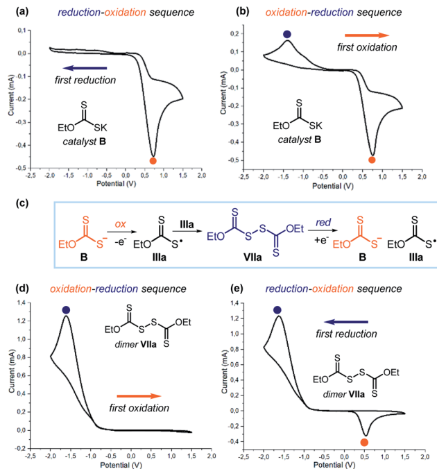
Fig. 11 Cyclovoltammetric studies of catalyst B [0.02 M] in [0.1 M] TBAPF 6 in \text{CH}_3\text{CN} : (a) reduction-oxidation scan sequence; (b) oxidation-reduction scan sequence. (c) The xanthyl radical IIIa, which can be formed by SET reduction of VIIa and oxidation of B, is the link between catalyst B and dimer VIIa. (d and e) Cyclovoltammetric studies of dimer VIIa [0.02 M] in [0.1 M] TBAPF 6 in \text{CH}_3\text{CN} : (d) oxidation-reduction scan sequence; (e) reduction-oxidation scan sequence. Sweep rate: 500 \text{ mV s}^{-1} . Pt electrode working electrode, Ag/AgCl (KCl 3.5 M) reference electrode, Pt wire auxiliary electrode.
