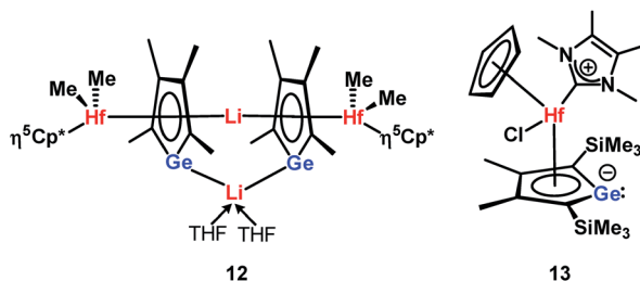
Fig. 4 Selected germole dianion metal complexes.
