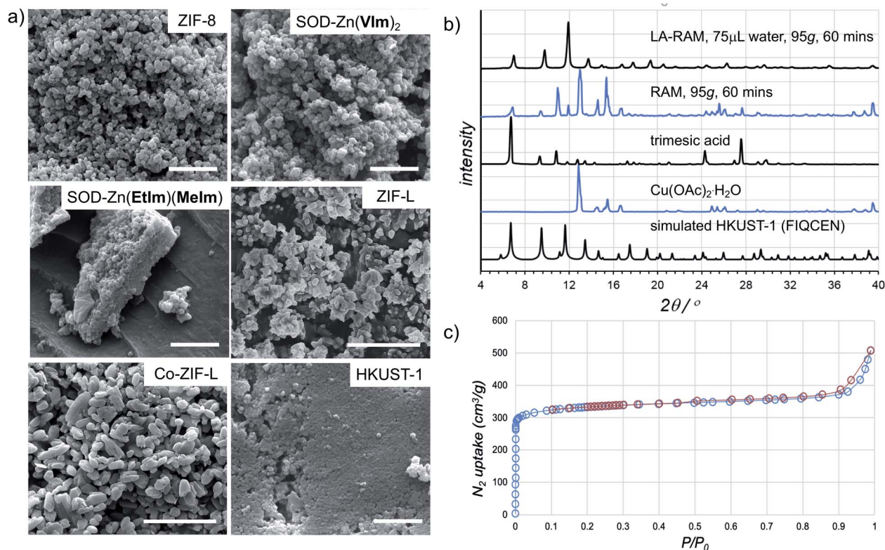
Fig. 4 (a) Example SEM images for samples of herein prepared MOFs (in each case, the bar corresponds to 1 \mu\text{m} ). (b) Comparison of the PXRD patterns for HKUST-1 prepared by LA-RAM with water (1 hour, 95g) to the neat reaction mixture, and the patterns of reactants and a simulated one for the MOF structure (CSD code FIQCEN). PXRD patterns for other LA-RAM experiments are given in the ESI.† (c) Nitrogen desorption and adsorption curves for HKUST-1 prepared by LA-RAM with water, after washing and evacuation.
