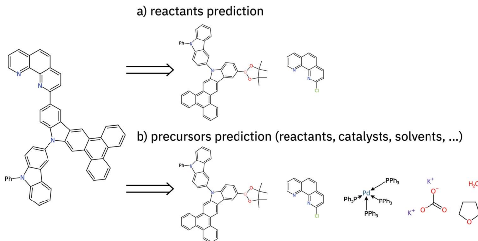
Fig. 1 Retrosynthesis step suggestion for 13-(1,10-phenanthrolin-2-yl)-10-(9-phenyl-9 H -carbazol-3-yl)-10 H -phenanthro[9,10- b ]carbazole using a chloro-Suzuki coupling reaction. In (a) only the reactants are predicted. In (b) all the precursors are predicted, which increases the overall difficulty of the single-step prediction task. While for (a) two molecules consisting of a total of 68 atoms are predicted, the target of (b) are six molecules consisting of 157 atoms.
