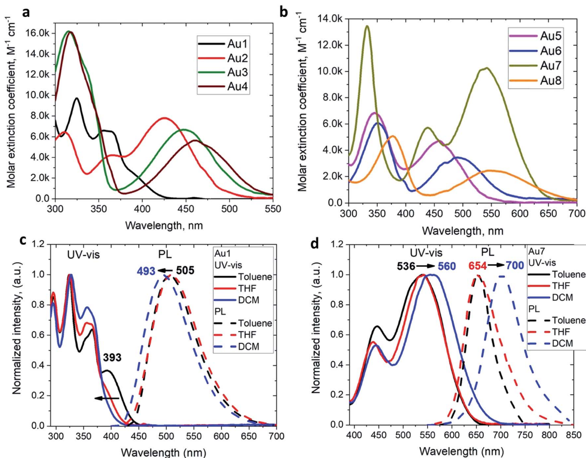
Fig. 3 UV-vis spectra of gold Au1–Au4 (a) and Au5–Au8 (b) complexes in THF solution (298 K). Normalized UV-vis and emission spectra in toluene, THF and CH_2Cl_2 for gold complex Au1 (c) and Au7 (d) showing negative and positive solvatochromism, respectively.
