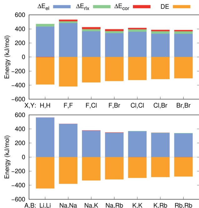
Fig. 4 Electrostatic ( \Delta E_{\text{el}} ), relaxation ( \Delta E_{\text{rlx}} ) and correlation ( \Delta E_{\text{cor}} ) contributions to the APOMO/RN-PP3 positron binding energy differences between e^+[X^-Y^-] and e^+[X^-] (top), and the CCSD(T) electron binding energy differences between e^-[A^+B^+] and A (bottom). The CCSD(T) dissociation energies (DE) for the [X^-Y^-] and [A^+B^+] systems are also given.
