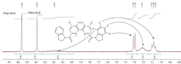
Fig. 12 ^1\text{H} NMR spectra of 3f in \text{DMSO}-d_6 at 55^\circ\text{C} (fragmental view).
