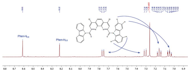
Fig. 13 ^1\text{H} NMR spectrum of 3h in \text{CDCl}_3 at 55^\circ\text{C} (region from 6.9 to 8.7 ppm).
