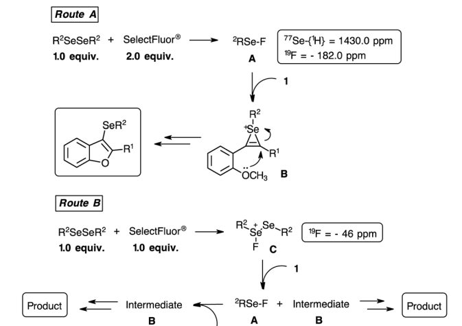
Scheme 7 Plausible mechanism routes for the synthesis of 3-organylselenanyl-benzo[b]furans 3.
