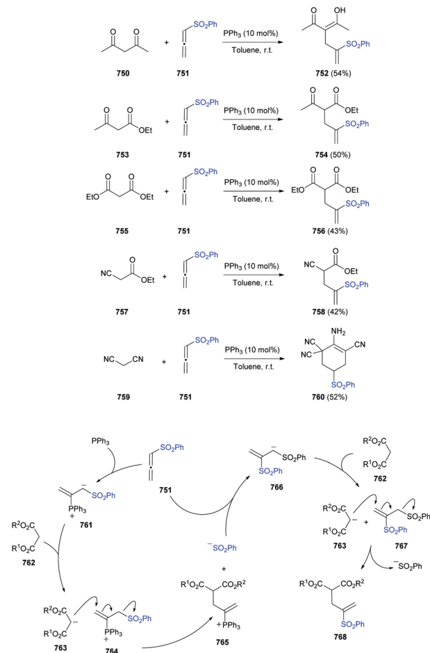
Scheme 112 Triphenylphosphine-catalysed 1,2-sulfonyl migration of electron-deficient allenes in their reaction with active methylene compounds affording vinyl sulfones.
